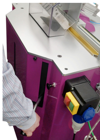
4 Cut the moulding - swing handle for angle, lift it to cut
